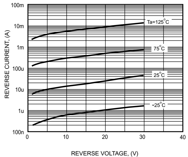
FIG. 4 - REVERSE CHARACTERISTICS
