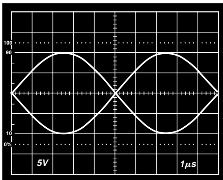
Figure 10. Driver 40 V p-p Differential Sine Wave; R_L = 50\Omega , f = 100kHz
