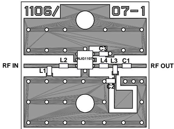
1.5/1.8/1.9GHz Band
