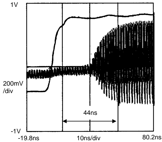
Switching speed ( V_{CTL1}=3.0V, V_{CTL2}=0V )
