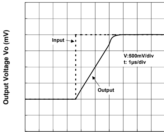
Slew Rate (Rise)
