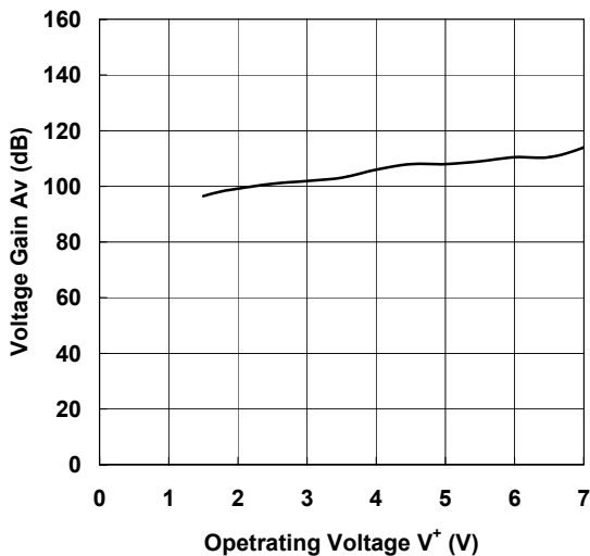
Voltage Gain vs. Operating Voltage (Ta=25°C, R_L=2k\Omega )
