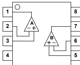
NJM12904D/12904M/12904E NJM12904V/12904R/12904RB1
