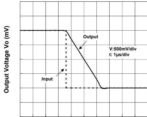
Slew Rate (Fall)
