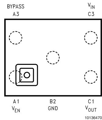
Top View See NS Package Number BPA05, BLA05, TLA05
