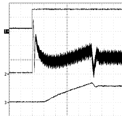
Start-Up: LM3500-16
