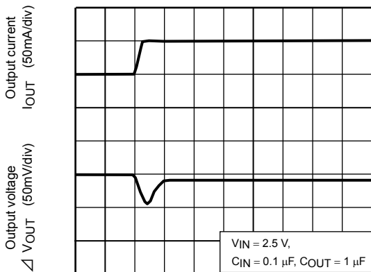
TCR5SB15 ( I_{OUT} = 50m to 100mA )
