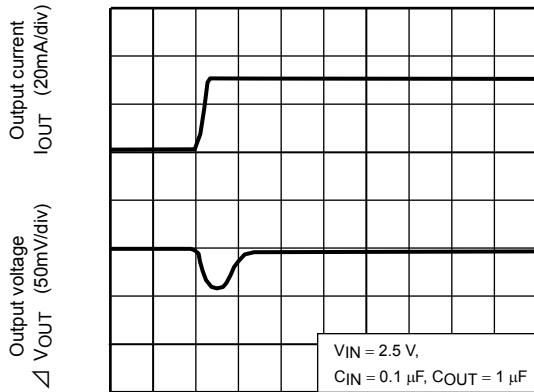
TCR5SB15 ( I_{OUT} = 1m to 30mA )
