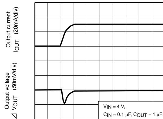
TCR5SB30 ( I_{OUT} = 1m to 30mA )
