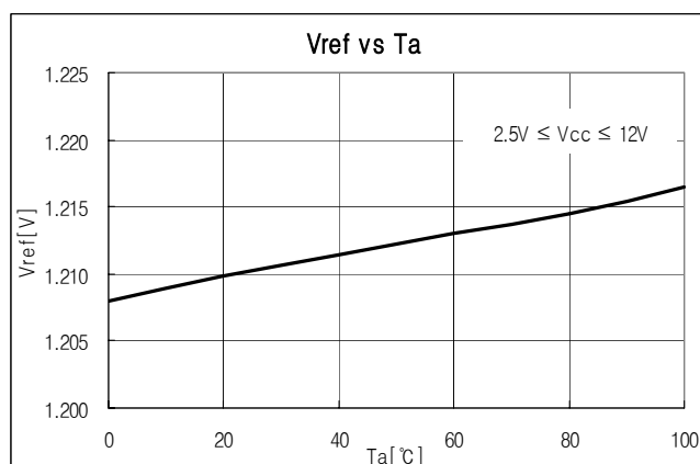
Fig.2 Vref vs Ambient Temperature
