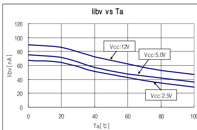
Fig.4 Vsense pin input bias current vs Ambient Temperature
