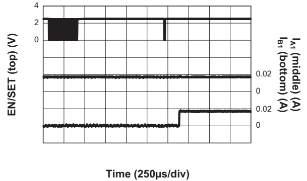
Transition of LED Current (Group B = 1.8mA to 20mA; Group A = 20mA)
