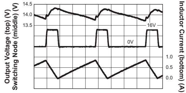
Output Ripple (All Channels = 20mA)
