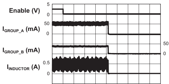
Shutdown Operation (All Channels)
