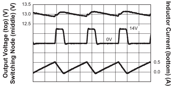
Output Ripple (All Channels = 10mA)
