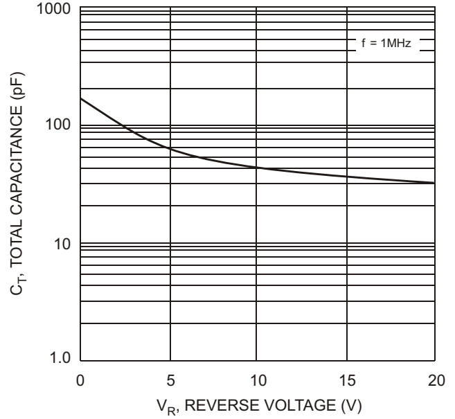
C_T , TOTAL CAPACITANCE (pF) V_R , REVERSE VOLTAGE (V) Fig. 4 Typ. Total Capacitance vs Reverse Voltage
