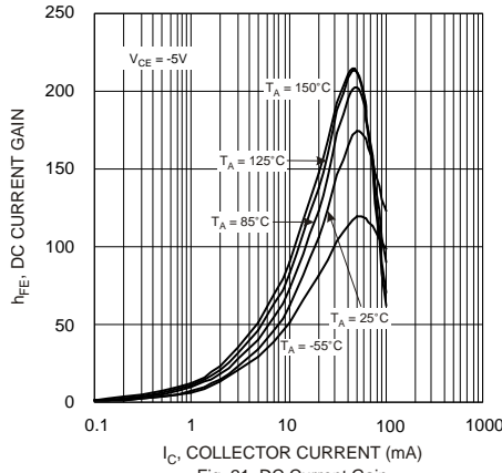
Fig. 21 DC Current Gain
