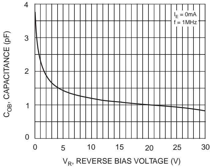
Fig. 28 Output Capacitance
