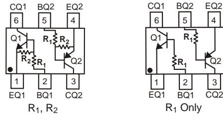
SCHMATIC DIAGRAM
