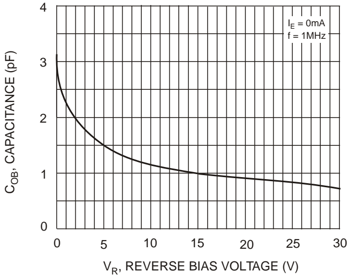
Fig. 9 Output Capacitance
