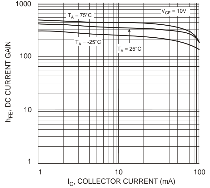
Fig. 32 DC Current Gain
