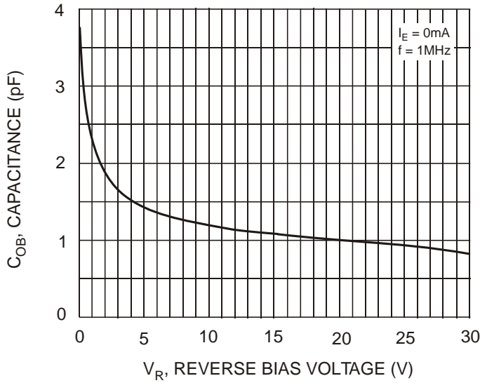
Fig. 33 Output Capacitance
