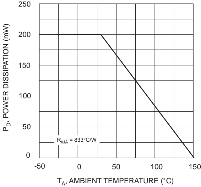
Fig. 1 Derating Curve
