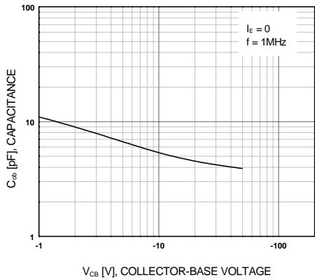
Figure 3. Output Capacitance
