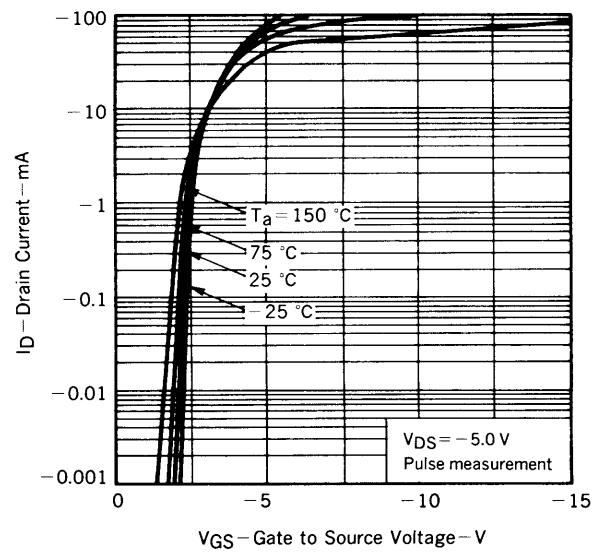
TRANSFER CHARACTERISTICS
