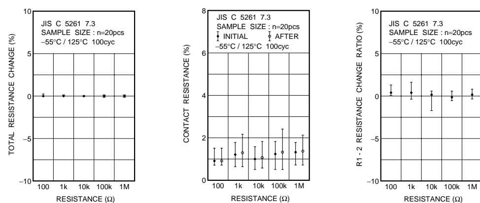
Fig.9 Temperature cycling
