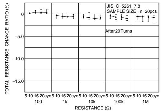
Fig.5-1 Endurance (wiper)
