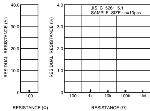
Fig.4 Residual resistance
