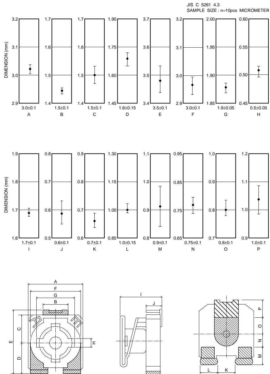
Fig.2 Dimensions
