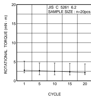
Fig.6 Rotational torque
