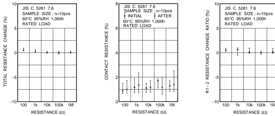
Fig.11 Endurance (under load in damp environment)
