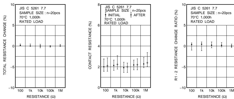
Fig.12 Endurance (rated load)
