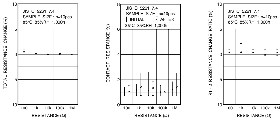
Fig.10 Resistance to humidity (steady state)
