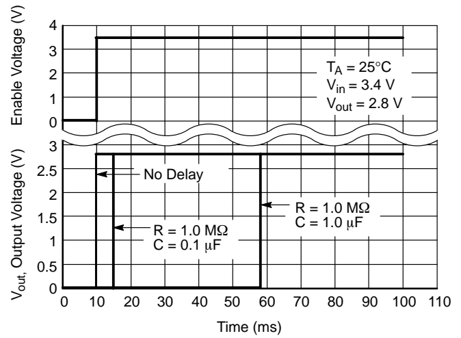
Figure 33. Delayed Turn-on
