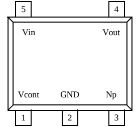
TK705xxS (SOT23-5)
