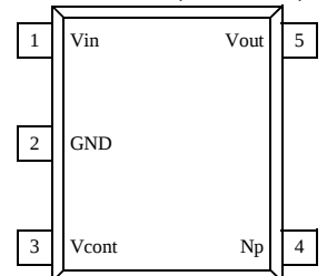
TK707xxS (SOT23-5)
