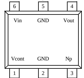
TK706xxH (SON2017-6)
