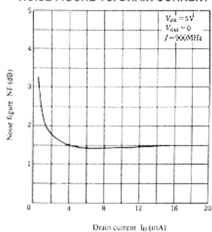
NOISE FIGURE VS. DRAIN CURRENT
