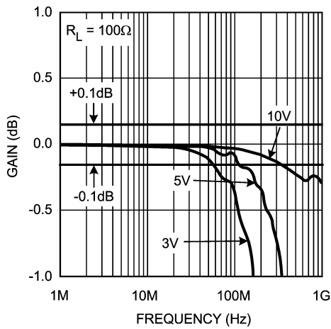
Gain Flatness
