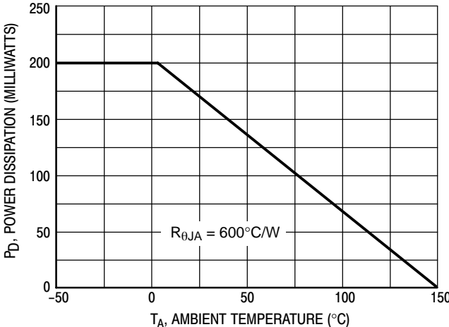
Figure 1. Derating Curve
