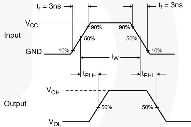
Figure 6. AC Waveforms
