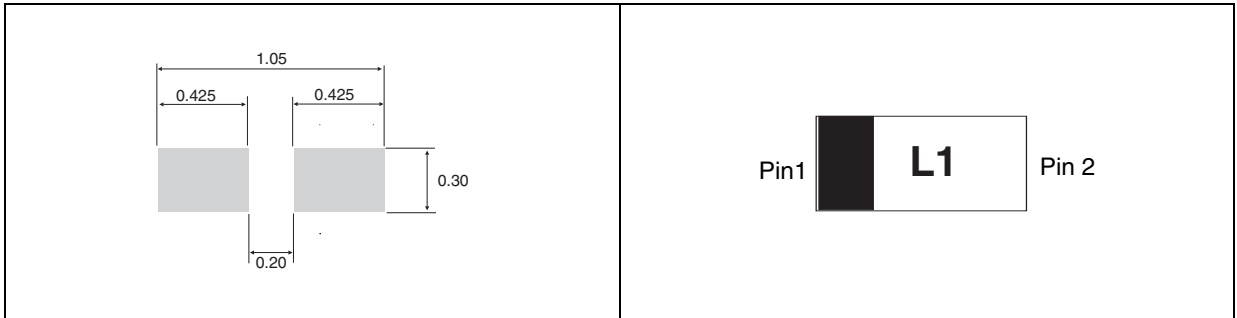
Figure 12. Footprint (dimensions in mm)
