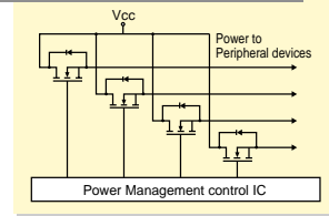
Power Management Circuit
