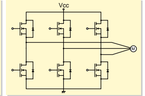
Motor Drive Circuit
