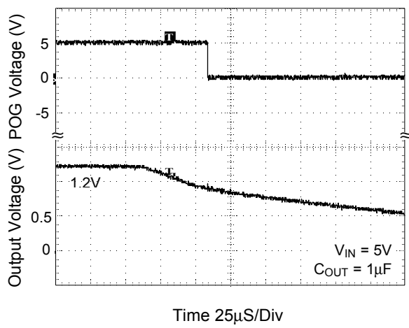
POG Response at Power Down
