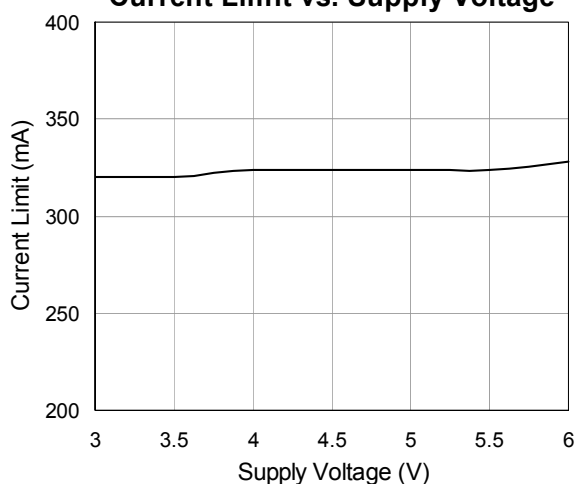
Current Limit vs. Supply Voltage
