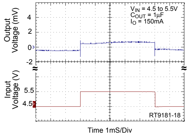
Line Transient
