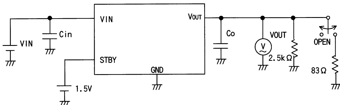
Fig. 5 Load Transient response (Characteristic example: Fig. 15~17)
