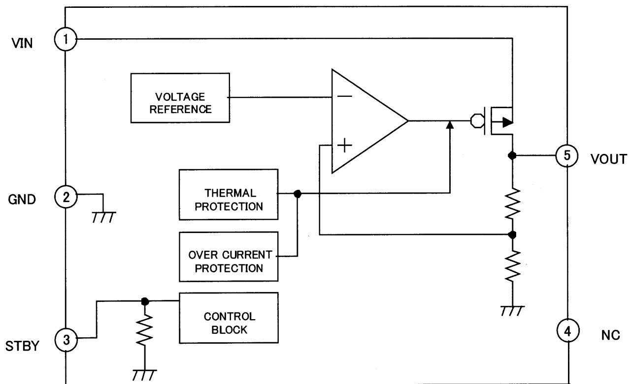
Fig.2 BLOCK DIAGRAM
