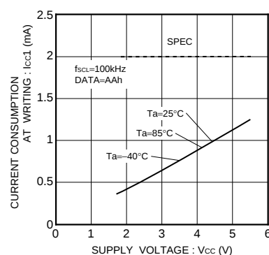
Fig.25 Write operating current I_{CC1} ( f_{SCL}=100\text{kHz} )
