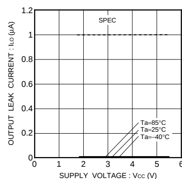
Fig.22 Output leakage current I_{LO}(\text{SDA})
