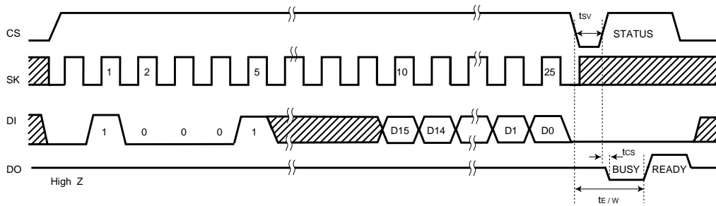
Fig.13 Write all address cycle timing. (WRAL)
