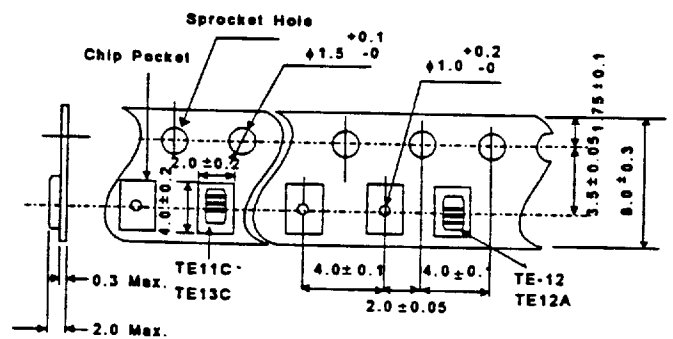
Tape and Reel Packing
