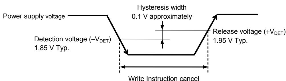
Figure 23 Operation at Low Power Voltage
