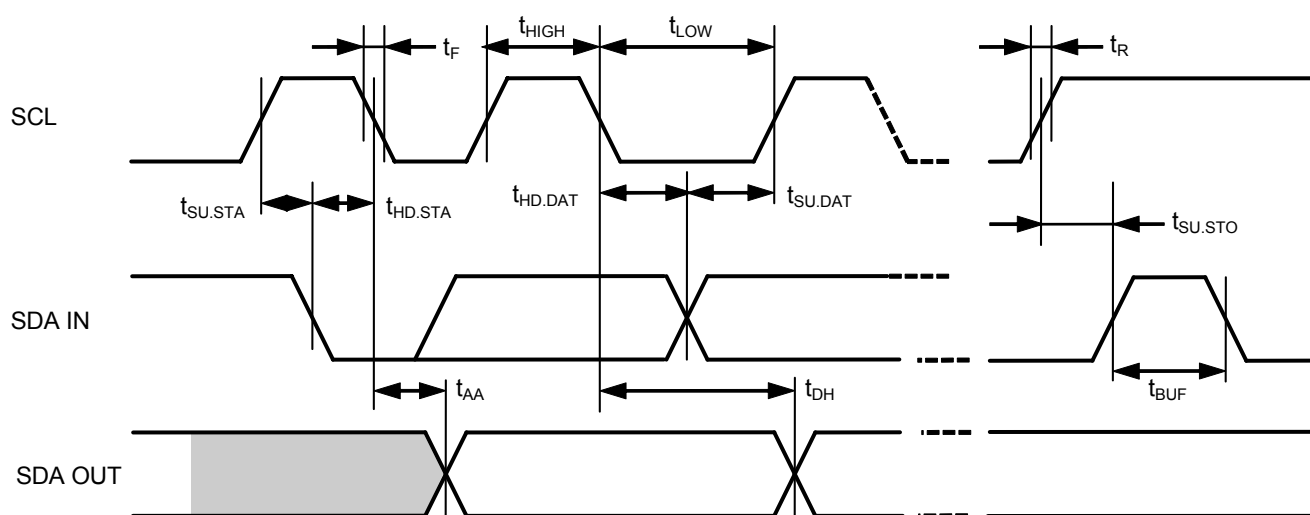
Figure 9 Bus Timing
