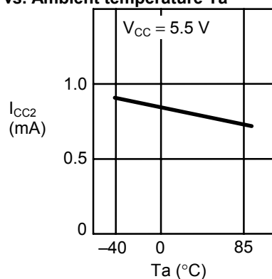
1. 9 Current consumption (PROGRAM) I_{CC2} vs. Ambient temperature T_a
