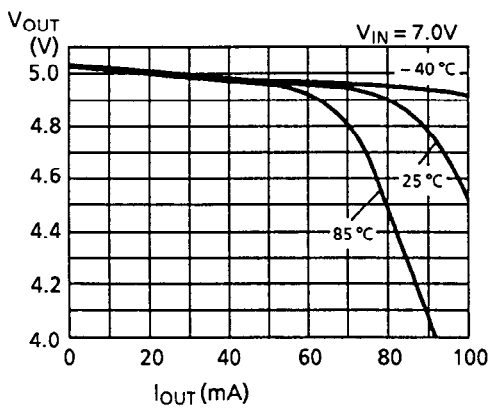
2.9 S-81250SG series
