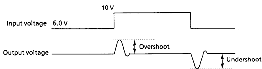
Figure 7 Output voltage fluctuation due to input voltage fluctuation
