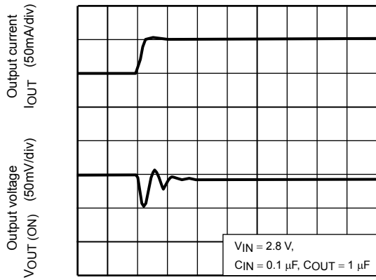
TCR5SB18A ( I_{OUT} = 50\text{m to }100\text{mA} )
