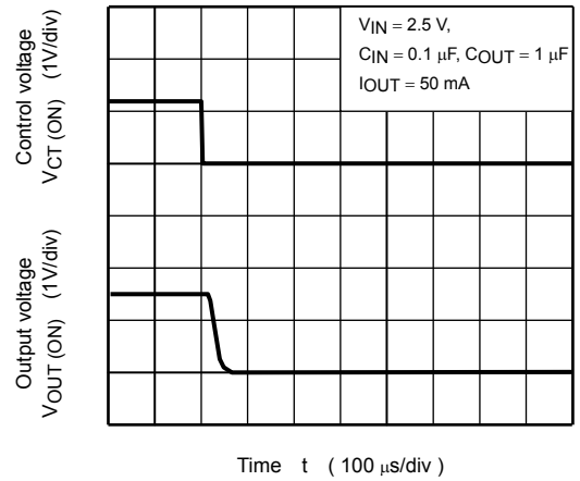
TCR5SB15A (Turn off wave form)
