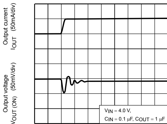
TCR5SB30A ( I_{OUT} = 50\text{m to }100\text{mA} )
