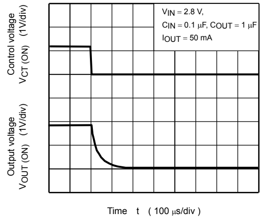
TCR5SB18A (Turn off wave form)
