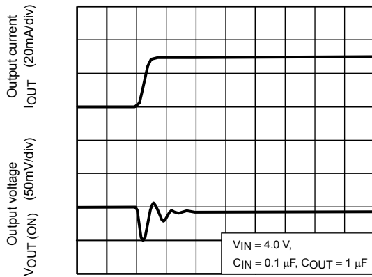
TCR5SB30A ( I_{OUT} = 1\text{m to }30\text{mA} )
