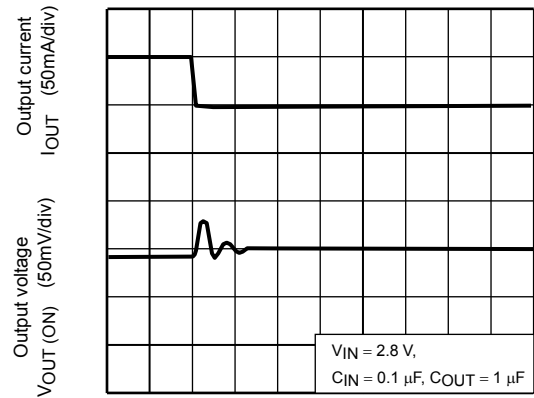
TCR5SB18A ( I_{OUT} = 100\text{m to }50\text{mA} )
