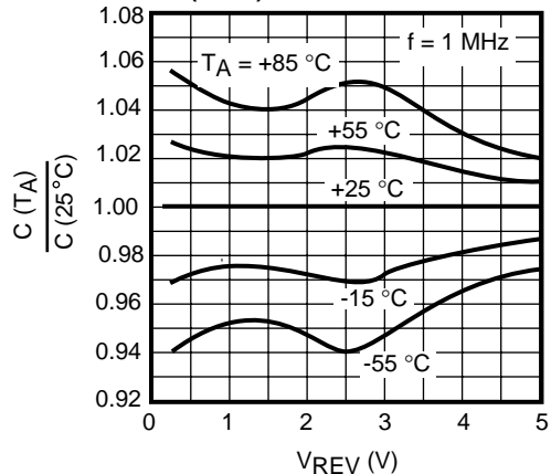
\frac{C(T_A)}{C(25^\circ\text{C})} vs. REVERSE VOLTAGE
