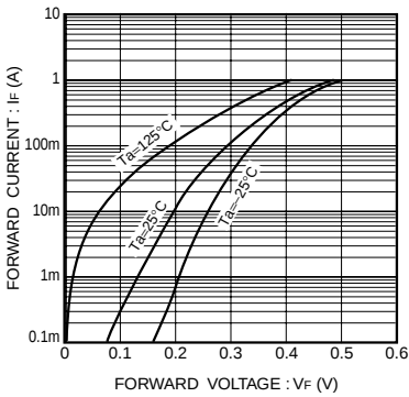
Fig.9 Forward characteristics
