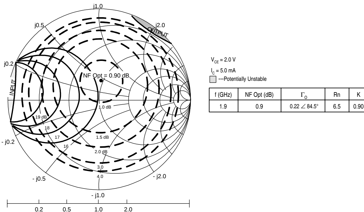
Figure 24. Constant Gain and Noise Figure Contours (f = 1.9 GHz)
