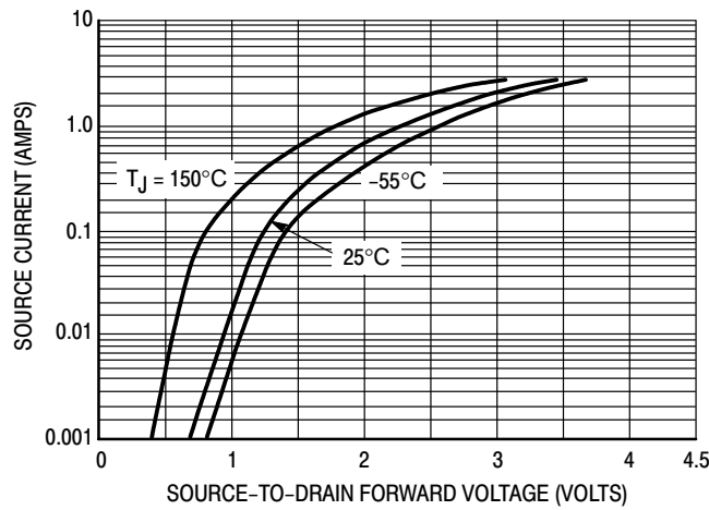
Figure 9. Source-to-Drain Forward Voltage versus Continuous Current (I S )
