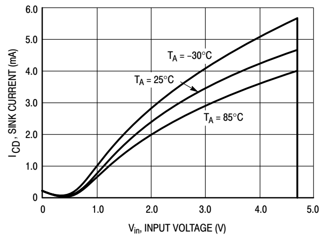
Figure 31. NCP302/3 Series 4.5 V C D Pin Sink Current versus Input Voltage
