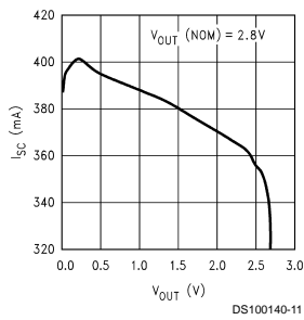
Short Circuit Current vs Output Voltage
