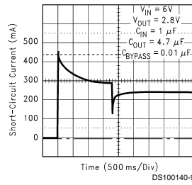
Short-Circuit Current
