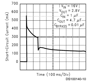
Short-Circuit Current
