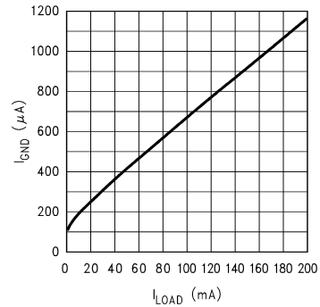
Ground Pin Current vs Load Current
