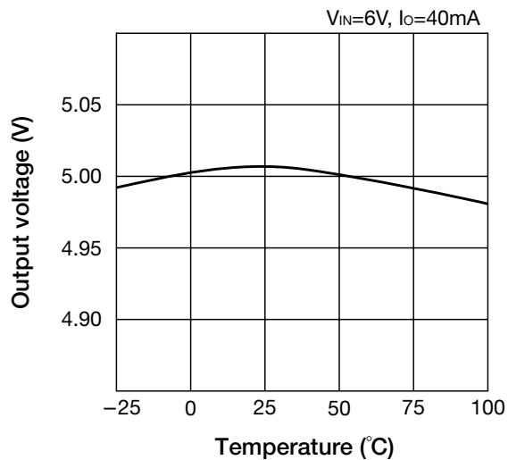
■ Output voltage temperature characteristic
