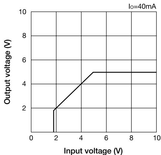
■ Output voltage characteristic
