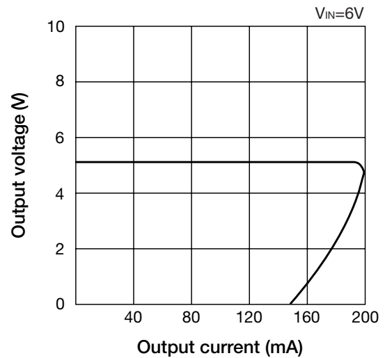
■ Output current characteristic
