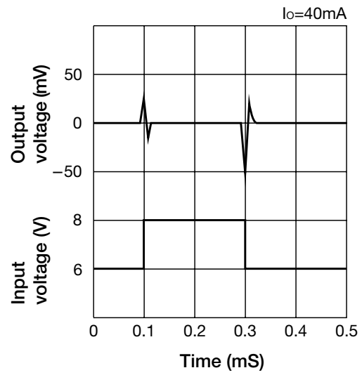
■ Transient response to input fluctuation
