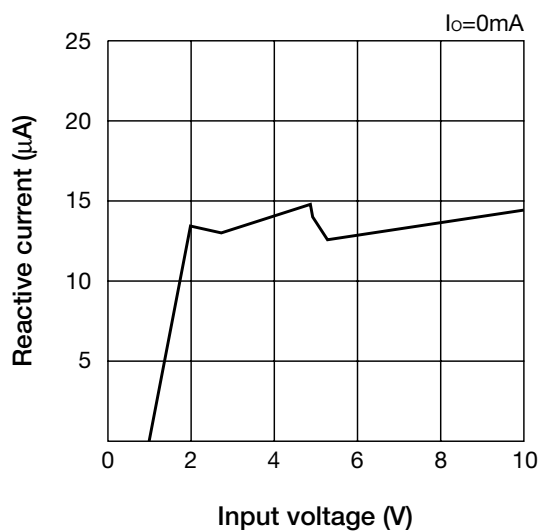
■ No-load input current
