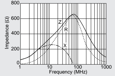
BLM31A601S
