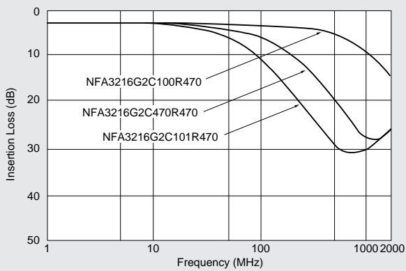
Resistance 47Ω line up
