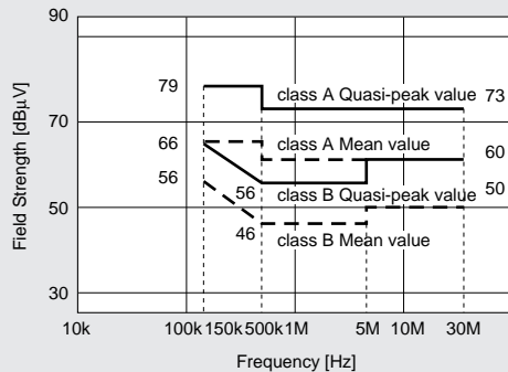
Radiated Interference
