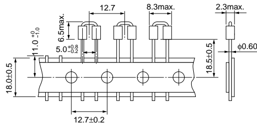
BL03RN2-R62T4
