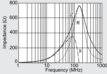
BLM31B601FI
