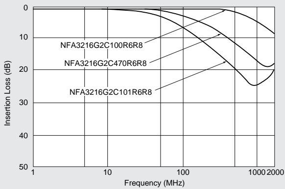
Resistance 6.8Ω line up
