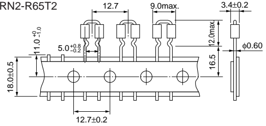
BL02RN2-R65T2
