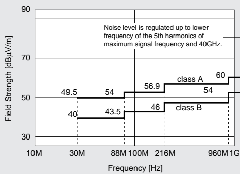
Radiated Interference
