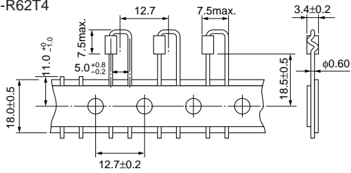
BL02RN2-R62T4
