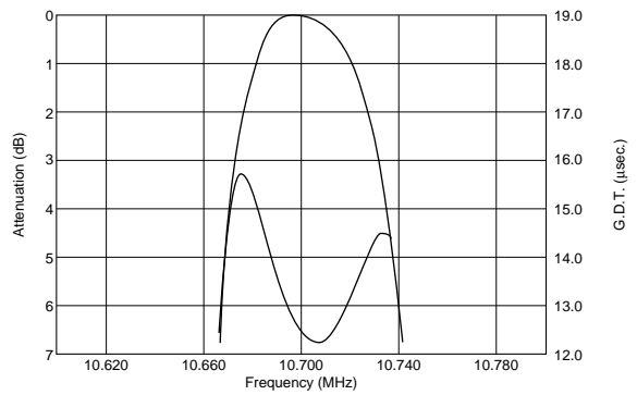
SFVLA10M7MF00-B0
