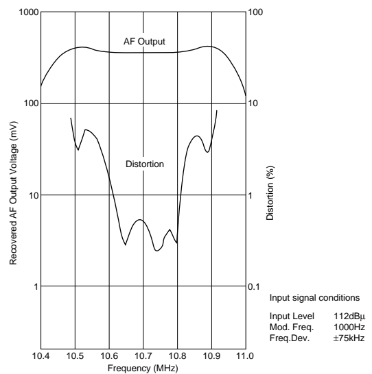
Frequency Characteristics
