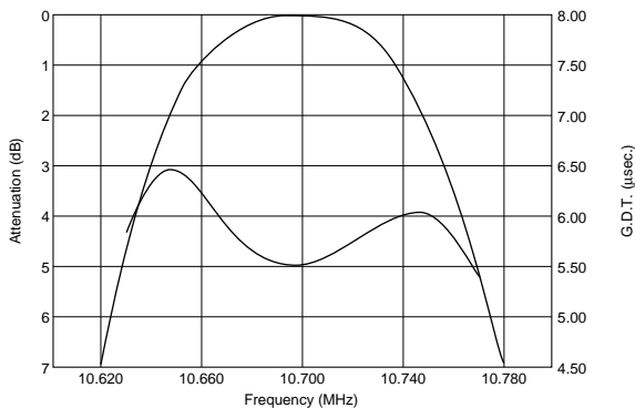
SFELA10M7KAH0-B0
