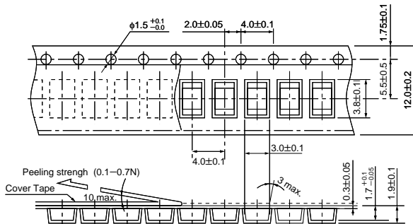
CDACV Series
