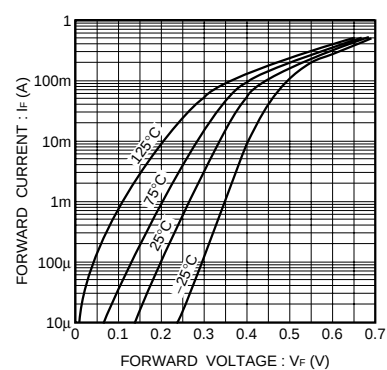
Fig.1 Forward characteristics
