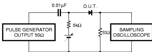
Fig. 6 Reverse recovery time (tr) measurement circuit
