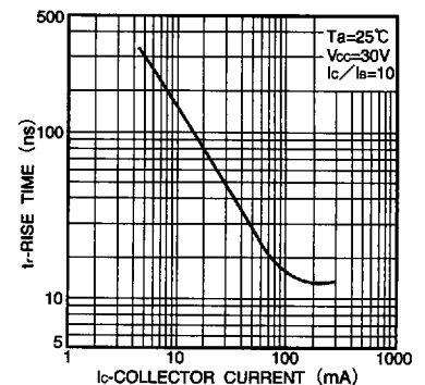
Fig.12 Rise time vs. collector current
