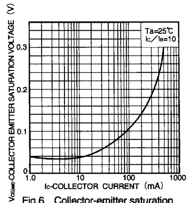
Fig.6 Collector-emitter saturation voltage vs. collector current
