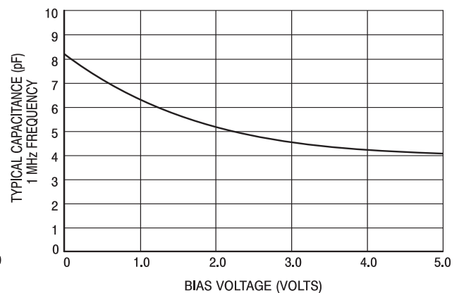
Figure 4. Capacitance
