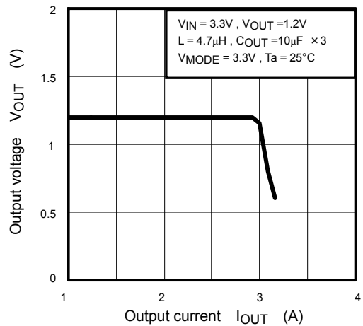
Overcurrent Protection (synchronous mode)
