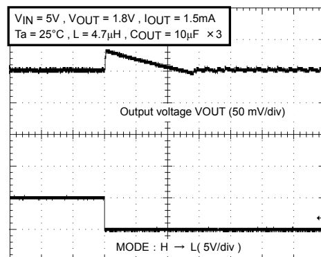
Mode Switching I_{OUT}=1.5mA (synchronous→non-synchronous)
