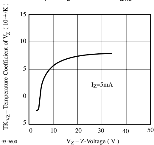
95 9600 Temperature Coefficient of V_Z vs. Z-Voltage
