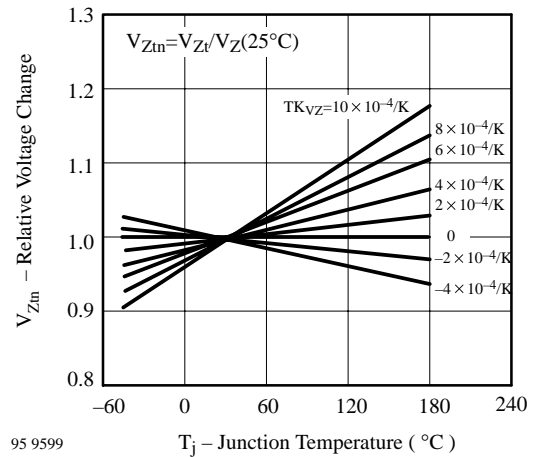
95 9599 Typical Change of Working Voltage vs. Junction Temperature
