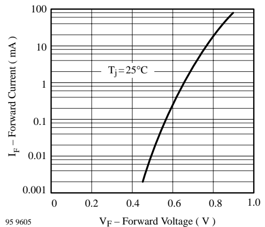
95 9605 Forward Current vs. Forward Voltage
