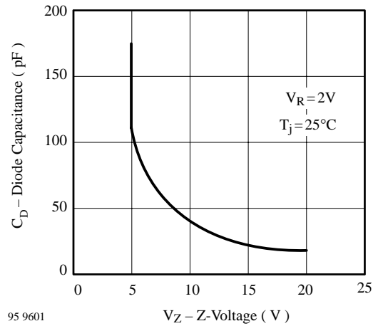
95 9601 Diode Capacitance vs. Z-Voltage
