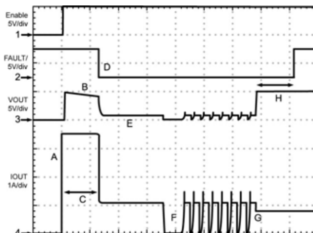
Figure 3. Kickstart Operation
