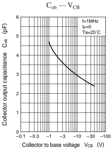
Characteristics charts of UN9117
